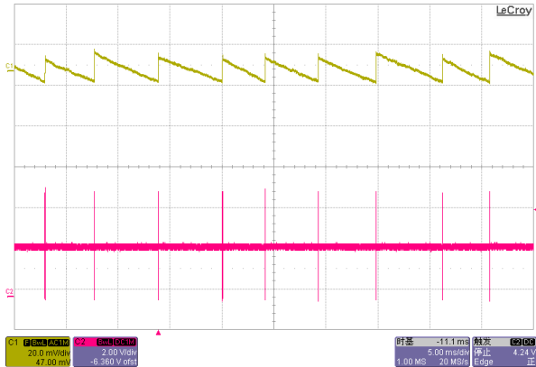
Output Ripple and SW at no load V_{in}=5V / V_{out}=2.5V
