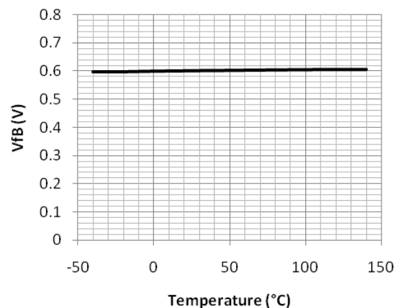
Vfb Vs. Temperature
