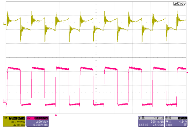
Output Ripple and SW at 1A load V_{in}=5V / V_{out}=2.5V
